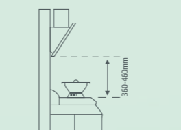
SLANTED HOOD
