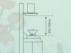
T-HOOD/ARCH-GLASS HOOD
