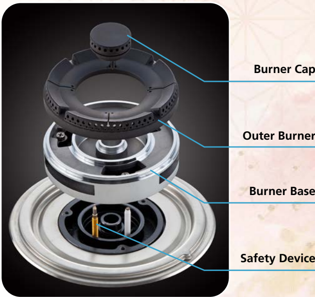
MBH-SD2112
