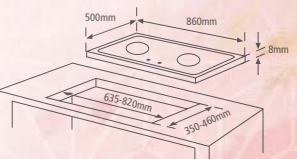
MBH-SD635 OPTIFLEX
