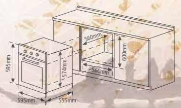
MBO-7680D
