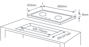
MBH-622 OPTIFLEX
