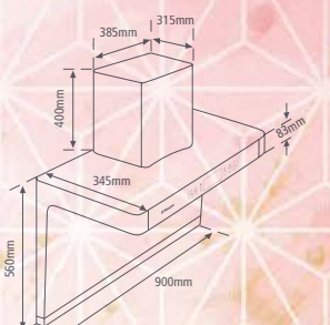
MDH-997MHC
