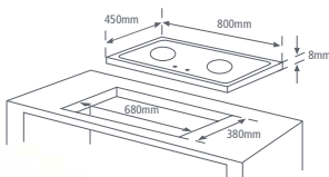
MBH-GC522C(BK) ROBUSTO
