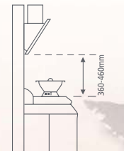
SLANTED HOOD
