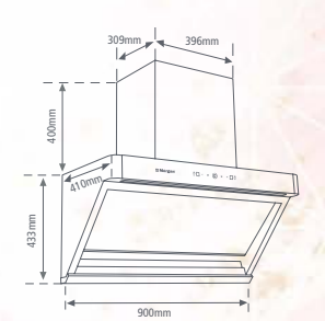
MDH-996MHC
