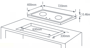
MBH-1665S
