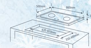
MBH-SD635 OPTIFLEX
