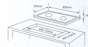
MBH-SD625 OPTIFLEX
