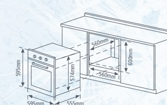
MBO-7680D
