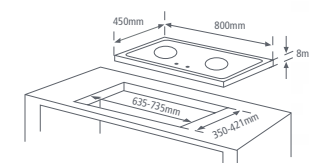
MBH-622 OPTIFLEX
