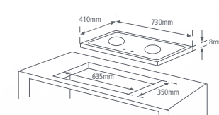
MBH-GC1142(BK)
